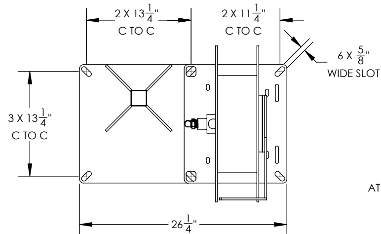
ANCHOR POINT DIMENSIONS WITH HOSE REEL EXPANSION
